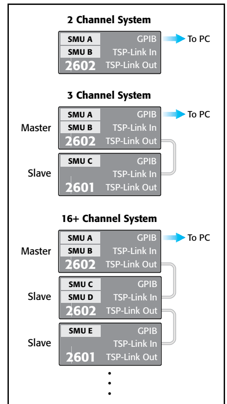
TSP-Link makes it easy to scale the system's channel count to match the application.
