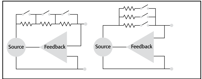
Series vs. parallel ranging topologies
